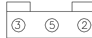
End View of 3-Pin Molex Connector
