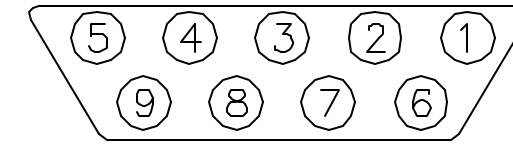
End View of 9-Pin Serial Port Connector
