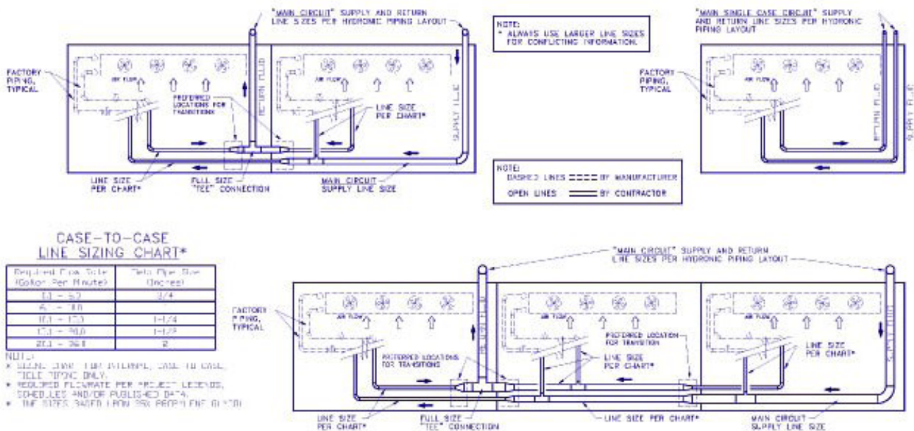
MEDIUM TEMPERATURE, SECONDARY COOLANT, INTERNAL CASE-TO-CASE PIPING DIAGRAM
