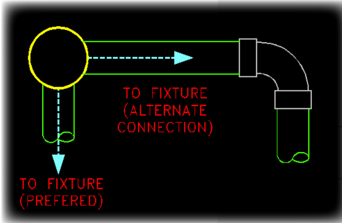
Branch Connections
