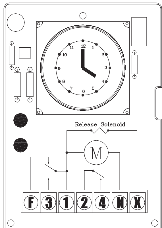
Defrost Timer
