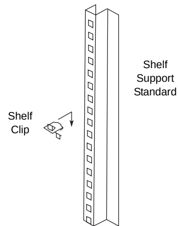
Shelf Installation
