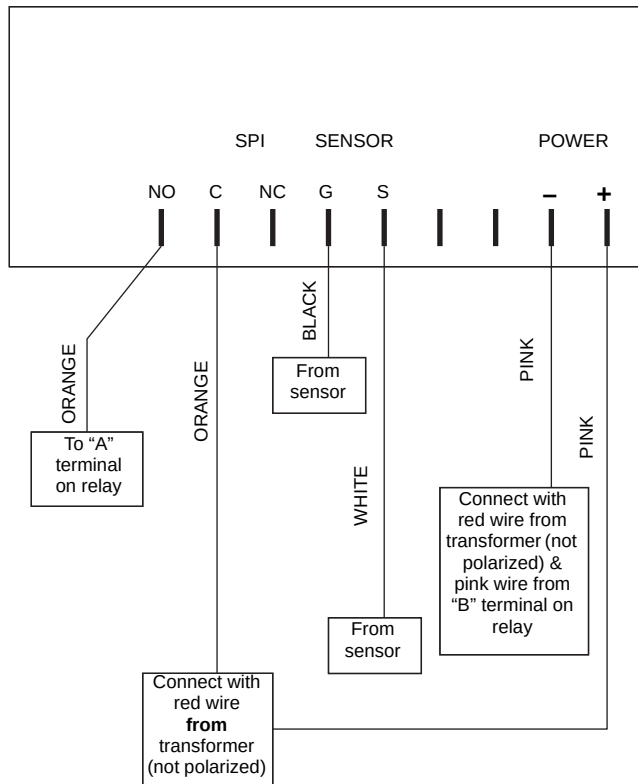
Digital Controller – Back View
