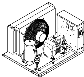
Indoor Unit
