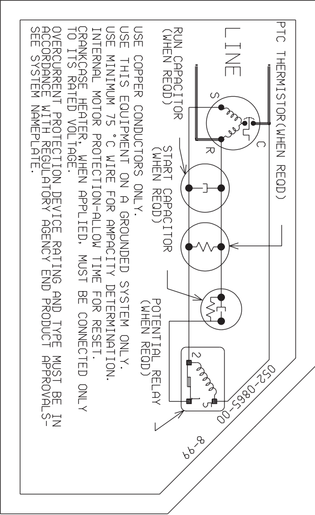
Wiring Diagram 0865
